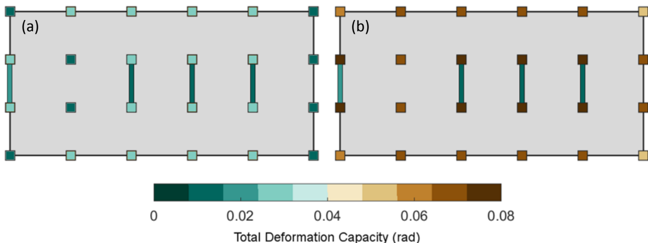
Figure 5 - Total deformation capacities in the backbone curves for the first-story walls and (a) the base of the first-story columns and (b) the top of the first-story columns.
