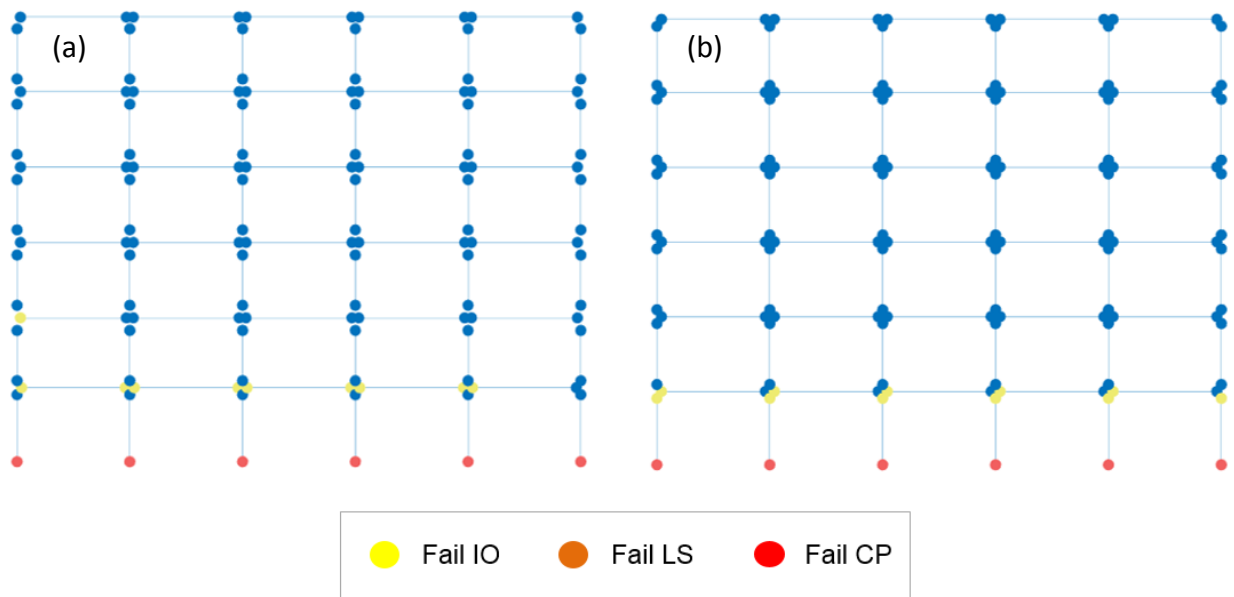
Figure 7 - Assessment of column and beam response relative to ASCE 41-17 nonlinear acceptance criteria for (a) exterior frame line 1 and (b) interior frame line 2.
