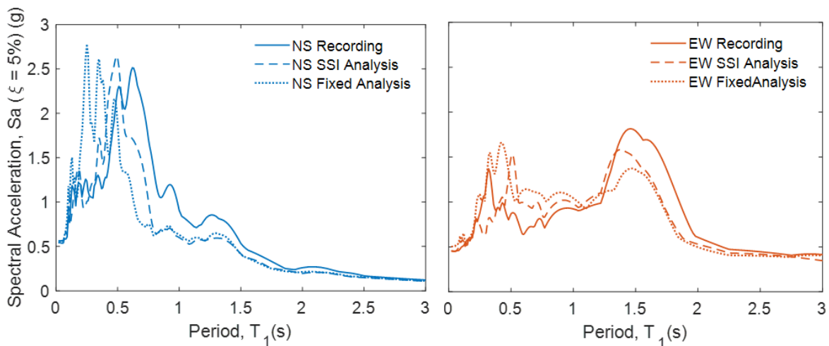
Figure 9 - Comparison of roof acceleration spectra from models with and without soil-structure-interaction. These spectra are computed from the accelerations recorded at the center of the roof in each direction.
